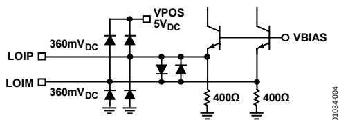
Figure 4. LO Port
