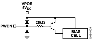
Figure 5. Power-Down Pin
